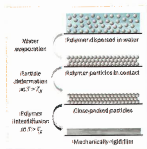
Figure 1—Formation of a film from a water dispersion of polymer nanoparticles.
