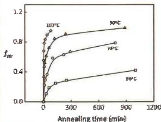
Figure 5 —Plots of f_m vs annealing time at different temperatures (56, 74, 90, 107°C) for latex films consisting of 1:1 ratio of Phe-PBMA and NBen(0.3)-PBMA latex particles.
