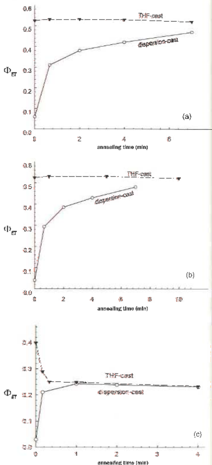
Figure 8—Evolution of \Phi_{ET} with annealing time in dispersion-cast and THF-cast films prepared from (a) Phe-PEHMA / Ant-PEHMA; (b) Phe-PEHMA / Ant-PEHMA-tBCEMA; and (c) Phe-PEHMA-MAA / Ant-PEHMA blends, annealed at 60°C.
