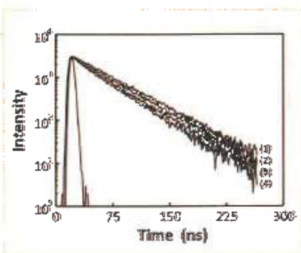
Figure 4 —Phenanthrene fluorescence decay profiles in PBMA latex films prepared from Phe-PBMA latex (1) and from a 1:1 ratio of Phe-PBMA and NBen-PBMA lattices (2-4), for a nascent film formed at room temperature (2), a film annealed for 60 min at 90°C (3), and a solvent-cast film (4).
