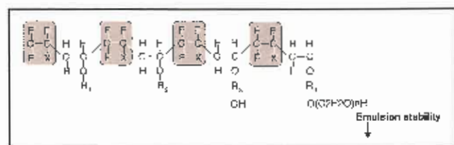
Figure 2—Polymer structure of FEVE emulsion.
