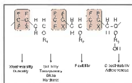
Figure 1—Polymer structure of FEVE copolymer.
