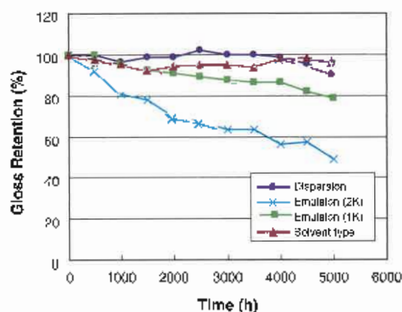
Figure 4—Accelerated weathering test result (QUV).
