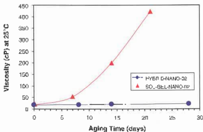
Figure 4—Comparison of viscosity changes as nanoparticle dispersion samples were aged at 60°C.
