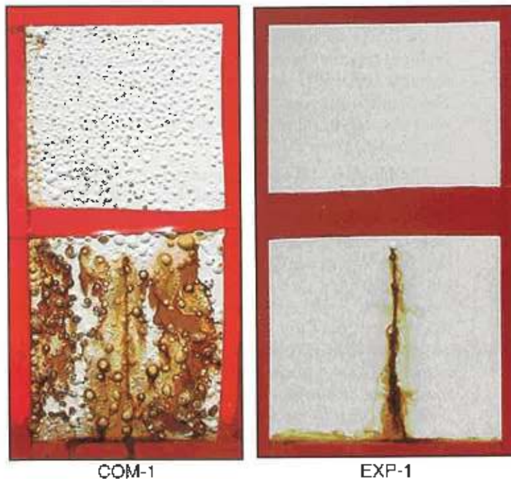
Figure 11. Steel panels after 35 days exposure to salt fog (ASTM B 117). Abrasive blasted hot rolled steel panels were coated with 3 mils DFT of 18 PVC gloss white DTM formulations, based on either EXP-1 or COM-1.
