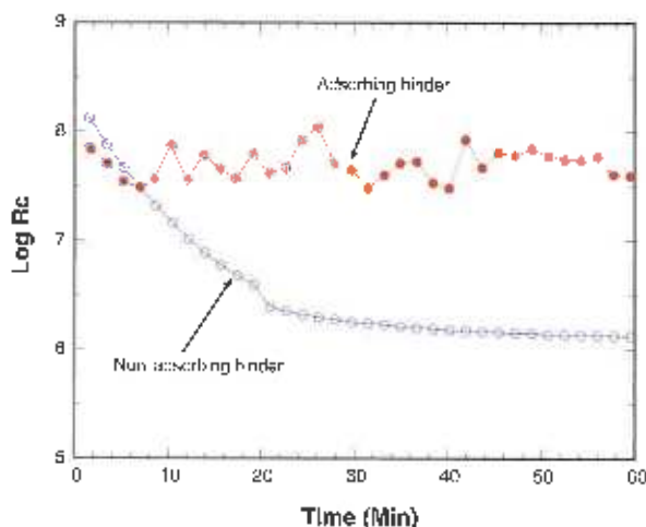
Figure 10—Plot of coating resistance ( R_c ) versus exposure time for 18 PVC DTM coatings based on adsorbing and non-adsorbing latex polymers. Data was derived from EIS measurements on films exposed to 5% NaCl solution.
