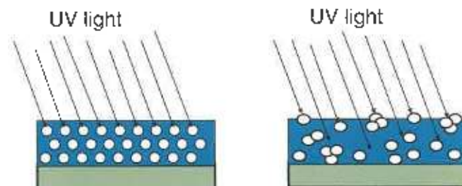
Figure 8—Representation of the interaction of UV light with coatings formed from adsorbing (left) and non-adsorbing (right) latex polymers; in particular, for coatings pigmented with titanium dioxide. The formation of polymer-pigment composites by the adsorbing polymer leads to improved \text{TiO}_2 dispersion in the dry film, which results in improved protection of the underlying polymer from UV light.
