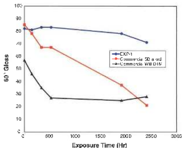
Figure 6—Plot of 60^\circ gloss versus exposure time for UV-A accelerated weathering comparing an 18 PVC gloss white DTM formulation based on polymer EXP-1 to commercial gloss white DTM coatings.
