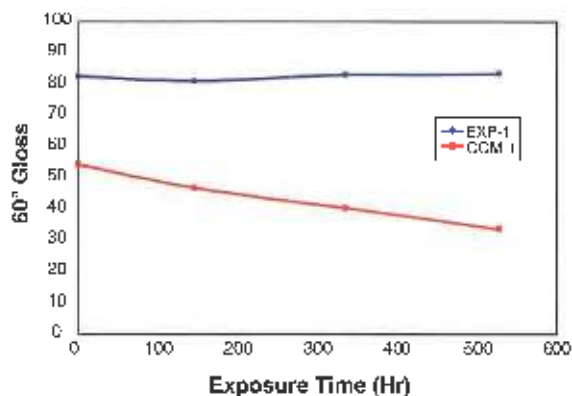
Figure 5—Plot of 60^\circ gloss values versus exposure time in UV-A accelerated weathering for 18 PVC paints based on adsorbing polymer EXP-1 and non-adsorbing polymer COM-1.
