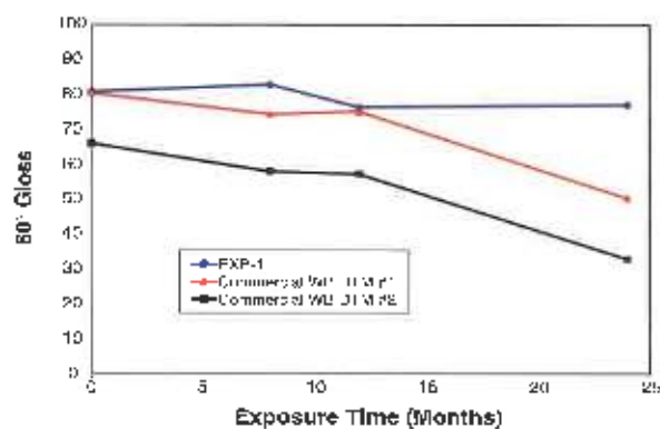
Figure 7—Plot of 60^\circ gloss versus exposure time for exterior exposures comparing an 18 PVC gloss white DTM formulation based on polymer EXP-1 to commercial gloss white waterborne acrylic DTM coatings. Panels were exposed south vertical at an eastern Pennsylvania site.
