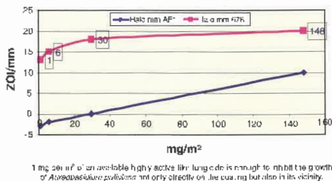
Figure 5—Activity of BCM and IPBC in a high PVC coating. The zone of inhibition (ZOI mm) is a measurement of activity against the test fungus Aureobasidium pullulans .
