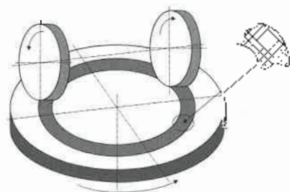
Figure 1—Taber test.
