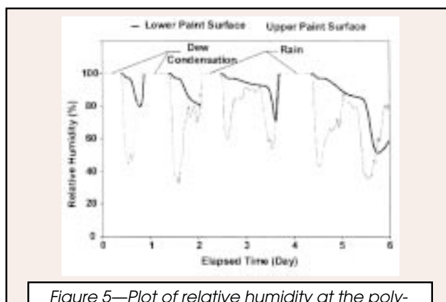
Figure 5—Plot of relative humidity at the polymer coating surfaces versus elapsed time for the illustrative six-day winter period in Miami, FL.
