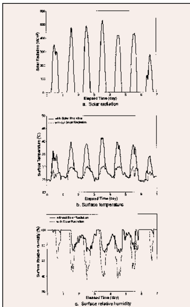
Figure 10—Illustration of the effect of solar radiation on surface temperature and surface relative humidity during first week of September in Miami, FL.
