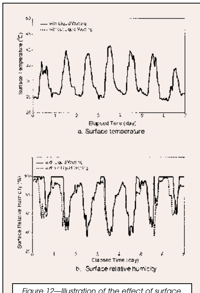
Figure 12—Illustration of the effect of surface wetting (rain and dew condensation) on surface temperature and surface relative humidity during the first week of September in Miami, FL. Note that in (a), the two curves overlap.
