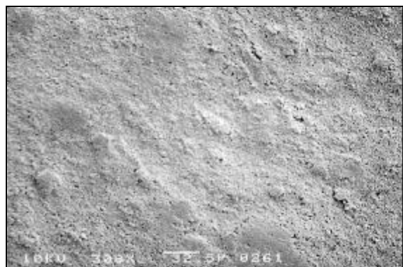
Figure 7—SEM of surface of SEAS-PVOH (103) coating.
