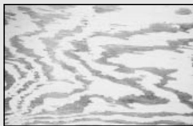
Figure 2—Paint failure over wide latewood bands on plywood.
