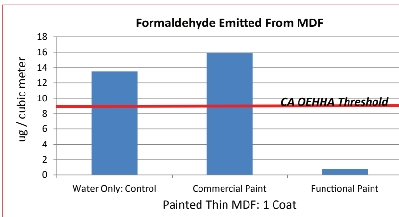
Figure 6 —Formaldehyde emissions from thin MDF samples that have one coat of various paints applied. Reference red line is the California's Office of Environmental Health Hazard Assessment cRel for formaldehyde exposure.
