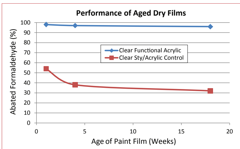
Figure 5 —Effectiveness of aged dry paint films at reducing formaldehyde in a microchamber with constant 1 ppmV spiked airflow.
