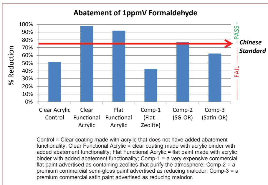
Figure 2 —Effectiveness of various dry paint films at reducing formaldehyde in a microchamber with constant 1 ppmV spiked airflow.
