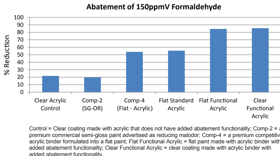
Figure 3 —Reduction of formaldehyde in chambers that contain various dried paint films and were injected with 150 ppmV.
