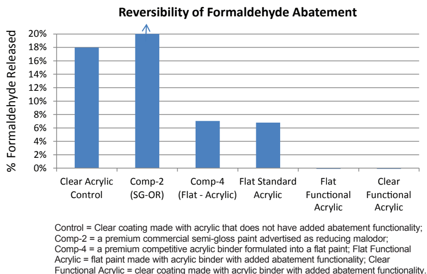
Figure 4 —Percent of formaldehyde abated during saturation which was determined to be released upon being placed into a clean environment.
