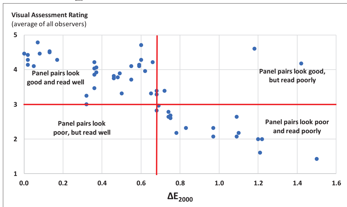
FIGURE 8—Visual ratings vs \Delta E_{2000} , with data placed into four quadrants.
