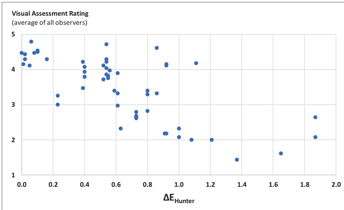
FIGURE 6—Visual Assessment Ratings vs \Delta E_{\text{Hunter}}
