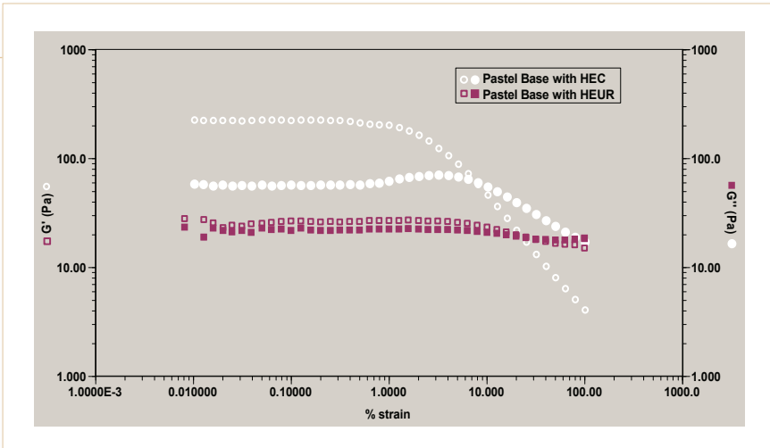
Figure 6 —Dependence of storage and loss moduli ( G' and G'' ) on % strain at 1 Hz frequency.
