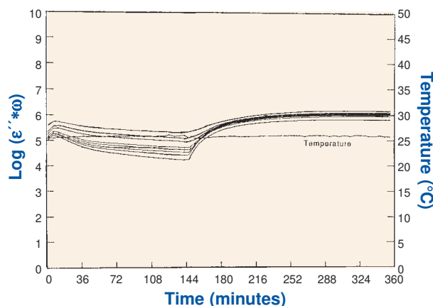
Figure 4—Similar measurement of coating cure where a second coat is applied at 144 min into cure.
