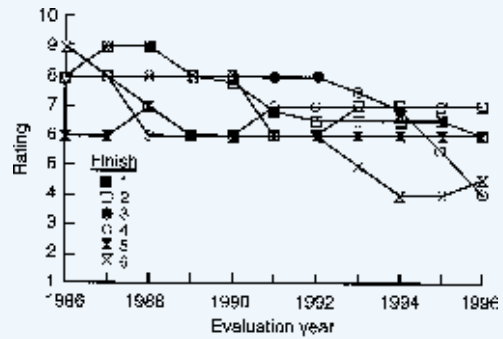
Figure 6—Average mildew rating for the finishes during 11 years (panels finished in 1985) of exterior exposure near Madison, WI. 10 = no degradation; 5 = point at which refinishing should be done; 1 = complete failure of finish (Finishes 1, 3, and 5 are alkyd based; Finishes 2, 4, and 6 are latex based).
