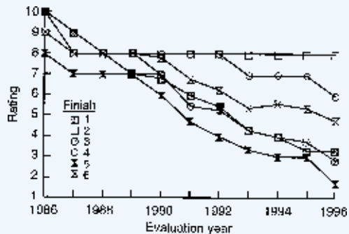
Figure 5—Average general rating for the finishes during 11 years (panels finished in 1985) of exterior exposure near Madison, WI. 10 = no degradation; 5 = point at which refinishing should be done; 1 = complete failure of finish (Finishes 1, 3, and 5 are alkyd based; Finishes 2, 4, and 6 are latex based).
