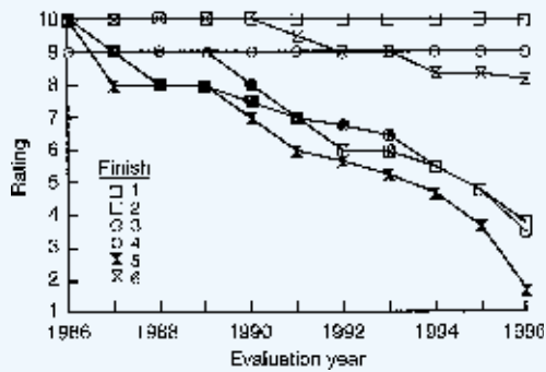
Figure 3—Average flaking rating for the finishes during 11 years (panels finished in 1985) of exterior exposure near Madison, WI. 10 = no degradation; 5 = point at which refinishing should be done; 1 = complete failure of finish (Finishes 1, 3, and 5 are alkyd based; Finishes 2, 4, and 6 are latex based).
