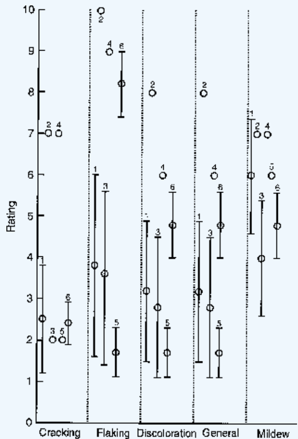
Figure 7—Comparison of mean ratings and standard deviations for Finishes 1 through 6 in each of the five evaluation categories after 11 years exterior exposure near Madison, WI (Finishes 1, 3, and 5 are alkyd based; Finishes 2, 4, and 6 are latex based).
