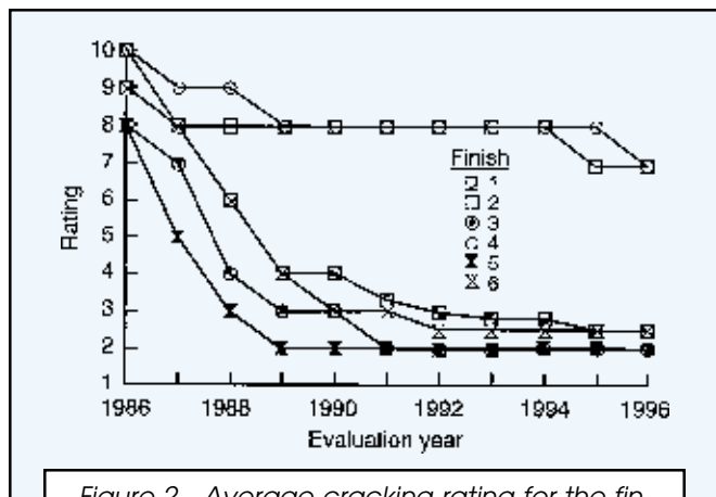
Figure 2—Average cracking rating for the finishes during 11 years (panels finished in 1985) of exterior exposure near Madison, WI. 10 = no degradation; 5 = point at which refinishing should be done; 1 = complete failure of finish (Finishes 1, 3, and 5 are alkyd based; Finishes 2, 4, and 6 are latex based).
