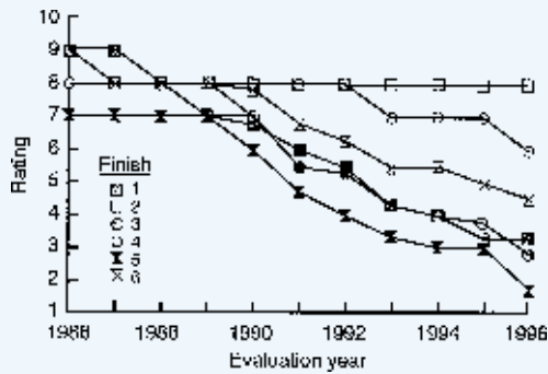
Figure 4—Average discoloration rating for the finishes during 11 years (panels finished in 1985) of exterior exposure near Madison, WI. 10 = no degradation; 5 = point at which refinishing should be done; 1 = complete failure of finish (Finishes 1, 3, and 5 are alkyd based; Finishes 2, 4, and 6 are latex based).
